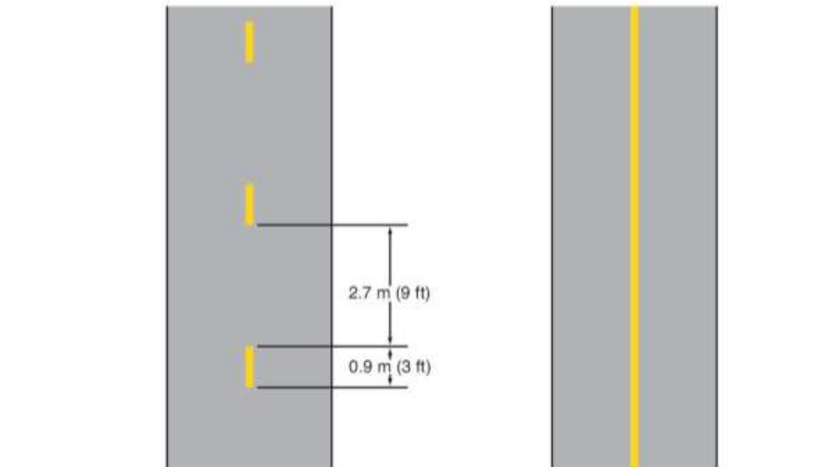
Figure 19: Examples of Centerline Markings for Trails
