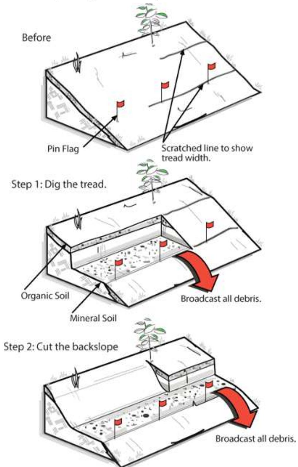
Figure 3: Typical MPOS Singletrack Full Bench Trail
